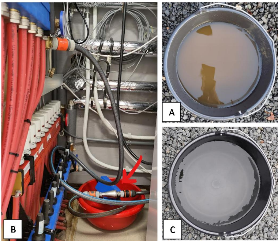
A: heating system water with rust fouling. B: Installation of vitalizer. C: heating system water three months after installation.
